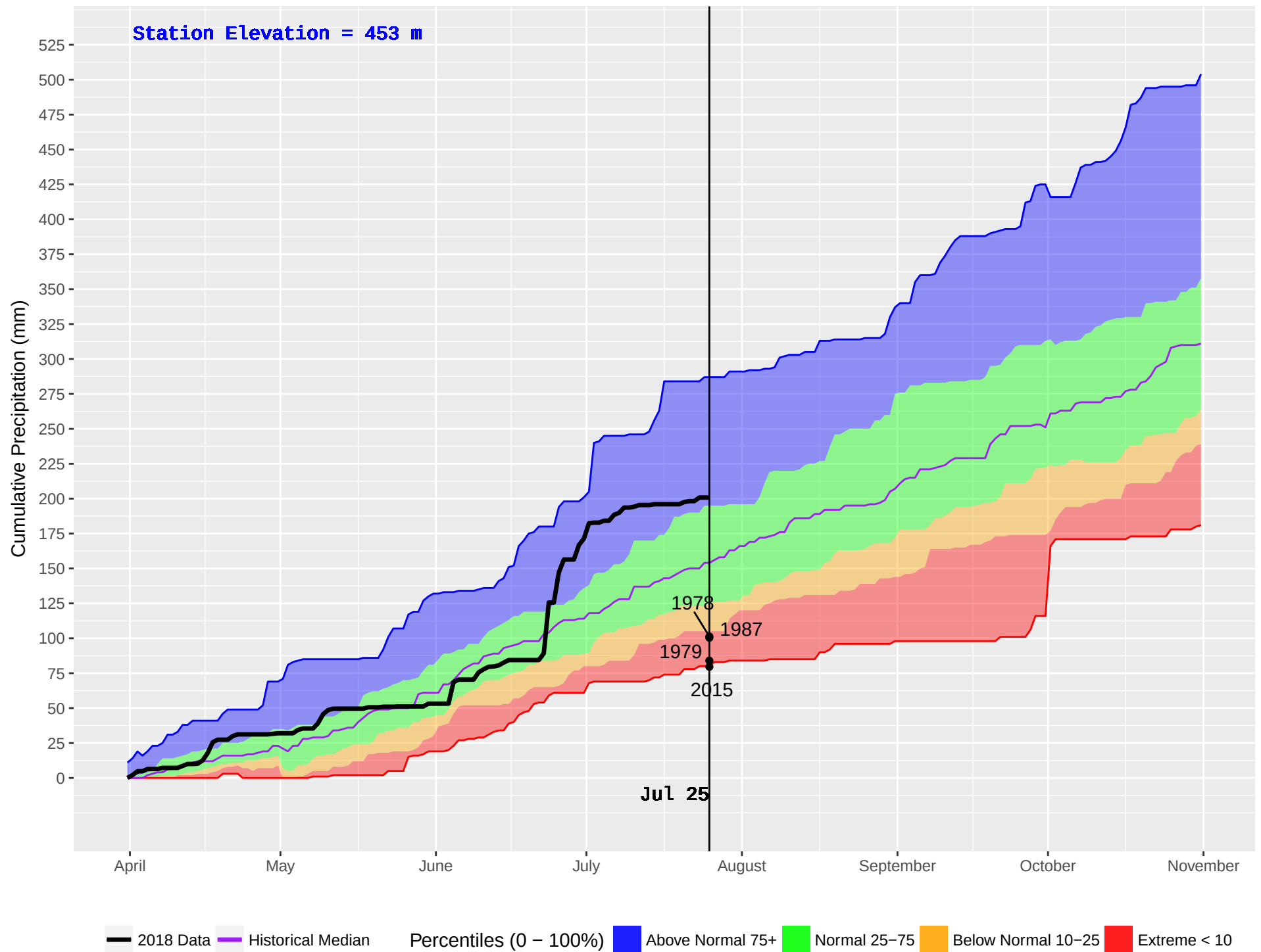
CLEARWATER HUB (239) : Historical (1976–2016) and Current (2018) Noon Cumulative Precipitation
