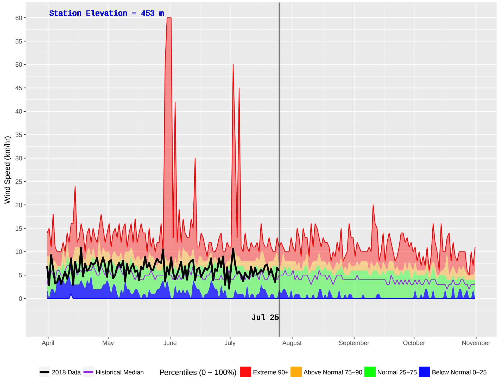
CLEARWATER HUB (239) : Historical (1976–2016) and Current (2018) Noon Wind Speed
