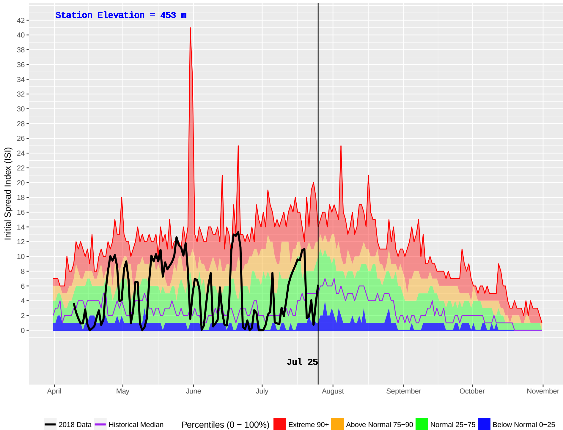
CLEARWATER HUB (239) : Historical (1976–2016) and Current (2018) Noon Initial Spread Index (ISI)
